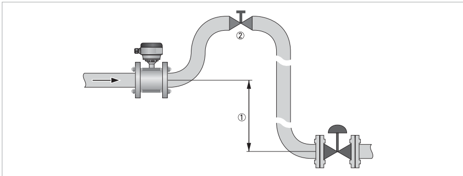
Figure 2-13: Air venting
