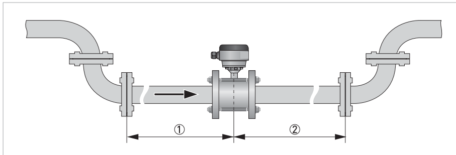
Figure 2-6: Recommended inlet and outlet section
