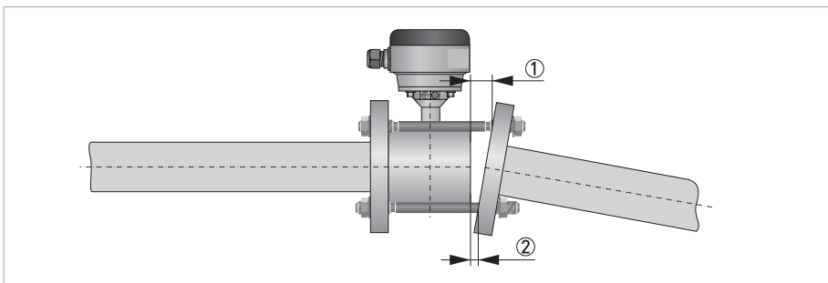
Figure 2-10: Flange deviation
