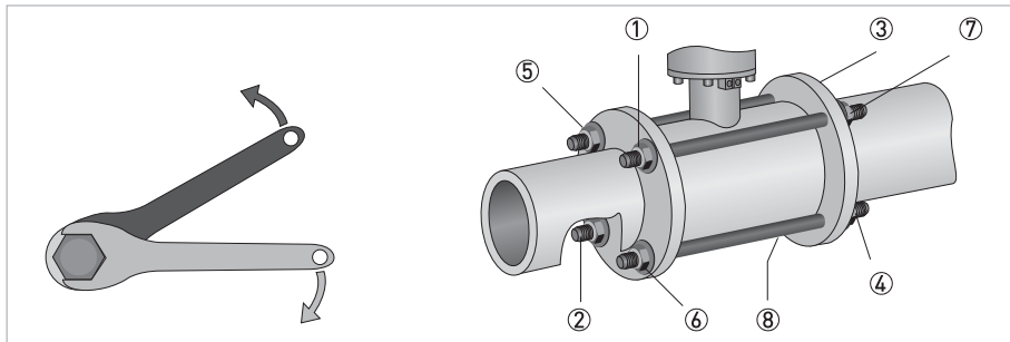
Figure 2-16: Tighten the bolts in fixed order, see picture.
