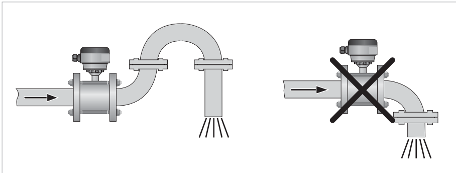
Figure 2-9: Installation in front of an open discharge
