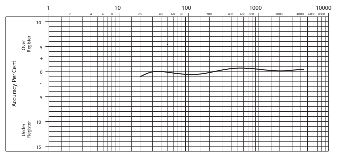
10 in. Meter
