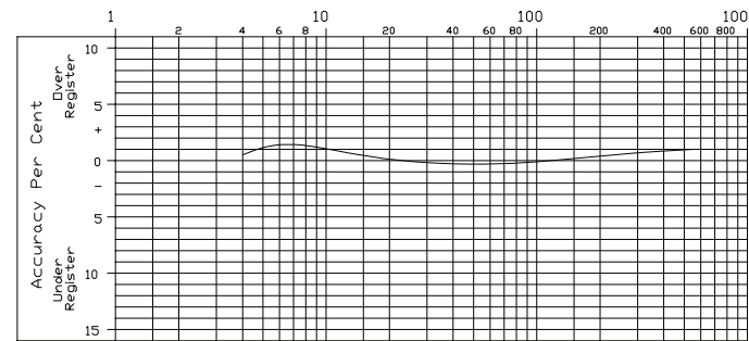
3 in. Meter
