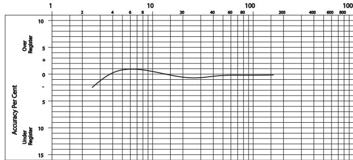
1-1/2 in. Meter
